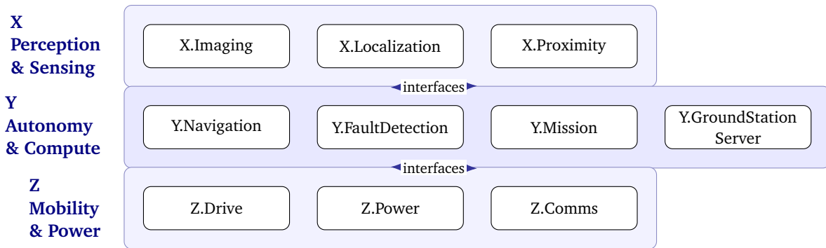
Figure 1: Three-layer architecture of the rover, showing each layer's subsystems
