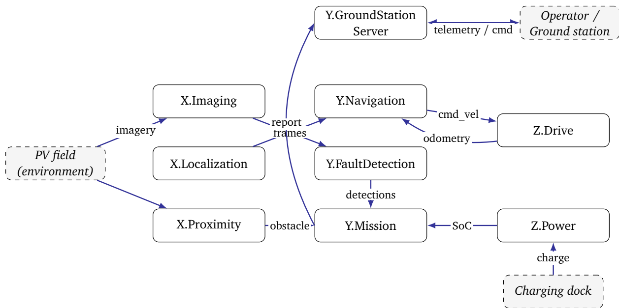
Figure 2: Subsystem data flow: sensing (X) → autonomy (Y) → mobility (Z), with the ground station and dock as external actors
